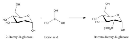
Figure 1. Chemical synthesis of Borono-Deoxy-D-glucose
